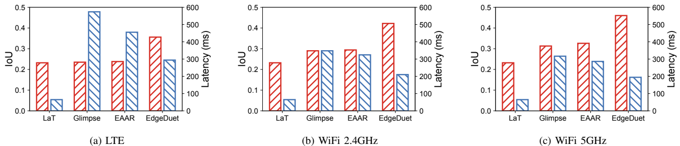
Fig. 9. End-to-end object detection accuracy (bars in red) and latency (bars in blue) of different methods under three network connections.
