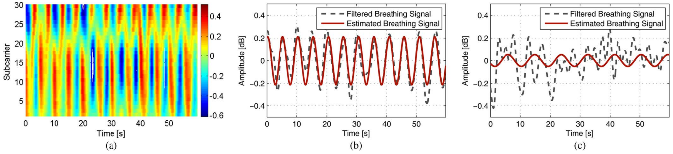
Fig. 9. Human breathing introduces diverse signal responses over different frequency subcarriers. (a) All subcarriers but a small portion (subcarrier #19~#24) depicts obvious breathing pattern, although the amplitude changes may be in the opposite direction (subcarrier #1~#19 vs. subcarrier #25~#30). (b) Estimated signals are remarkably close to the breathing signals when using subcarrier #10. (c) Incorrect frequency with meaningless amplitude may be resulted in if using subcarrier #24. (a) Breathing signals over all subcarriers. (b) breathing signals at subcarrier #5. (c) breathing signals at subcarrier #24.
