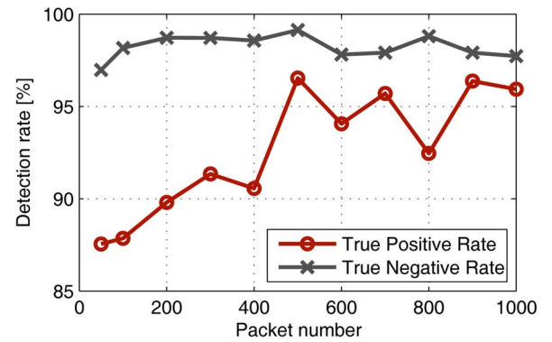
Fig. 13. Impacts of packet quantity on detection accuracy of moving target.
