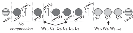
Figure 4: An illustration of the locations that different layer compression techniques are applied to AlexNet.
